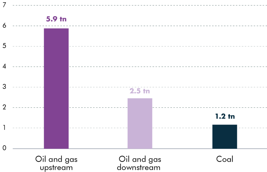
FIGURE 10 – FOSSIL FUEL SUPPLY INFRASTRUCTURE ASSET VALUE ($TN)
